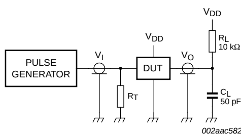
Fig 19. Test circuitry for switching times, \overline{INT}
